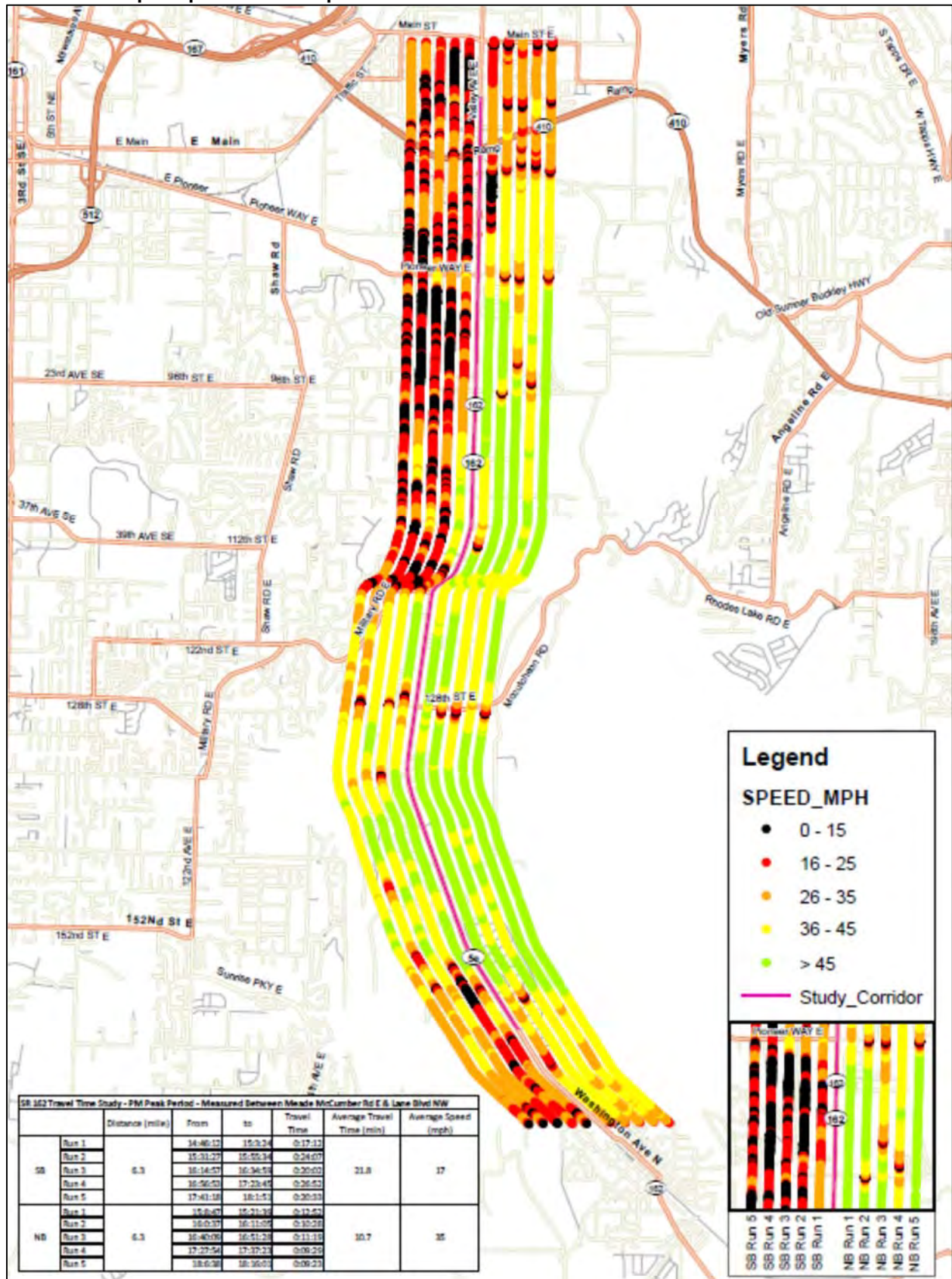
Exhibit 8: PM peak period travel speed
