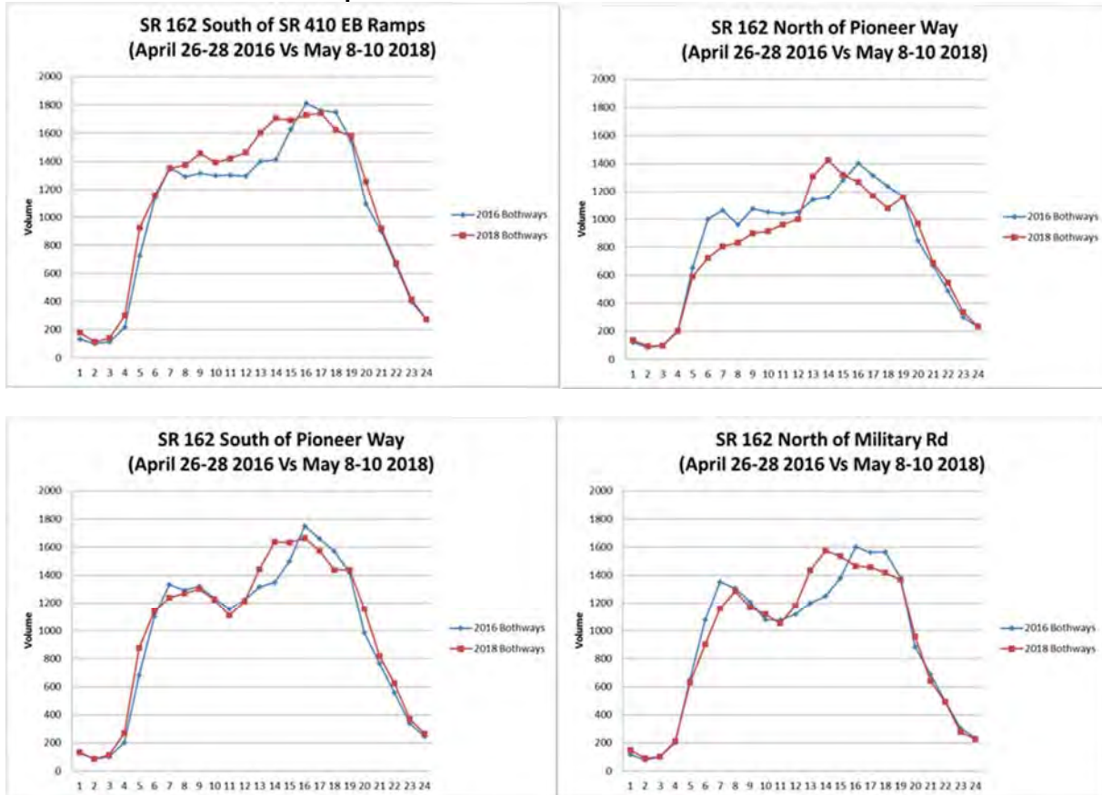
Exhibit 3: Traffic volume comparison between 2016 and 2018
